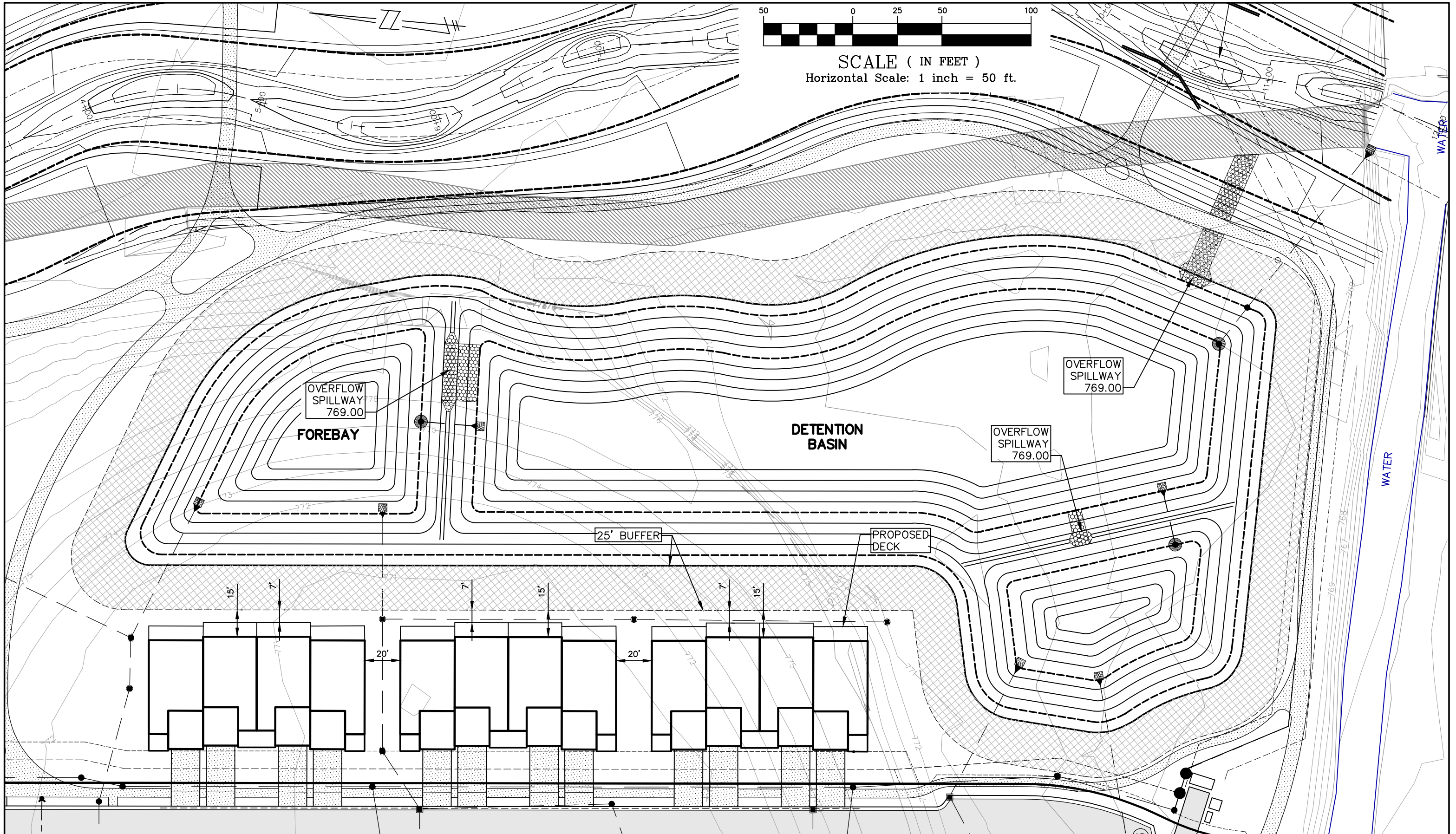
BASIN AND SIDEWALK LAYOUT
